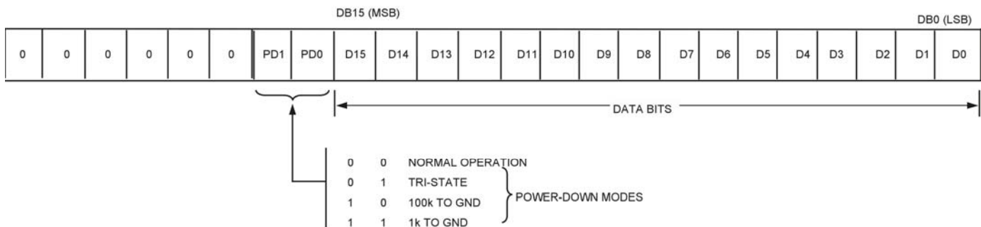
Figure 22. AD5060 Input Register Contents
